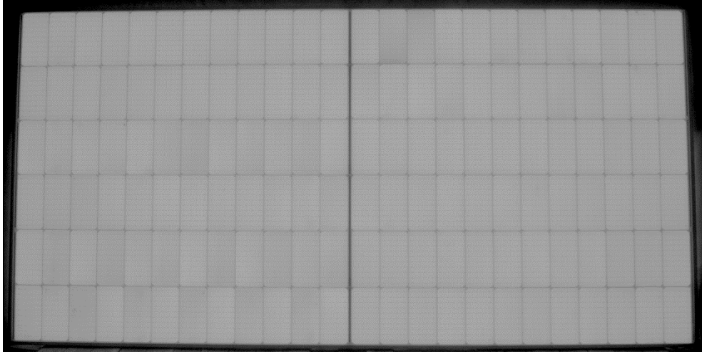
Fig. 7 EL photo of module No.1 Serial number: AS22191106794
