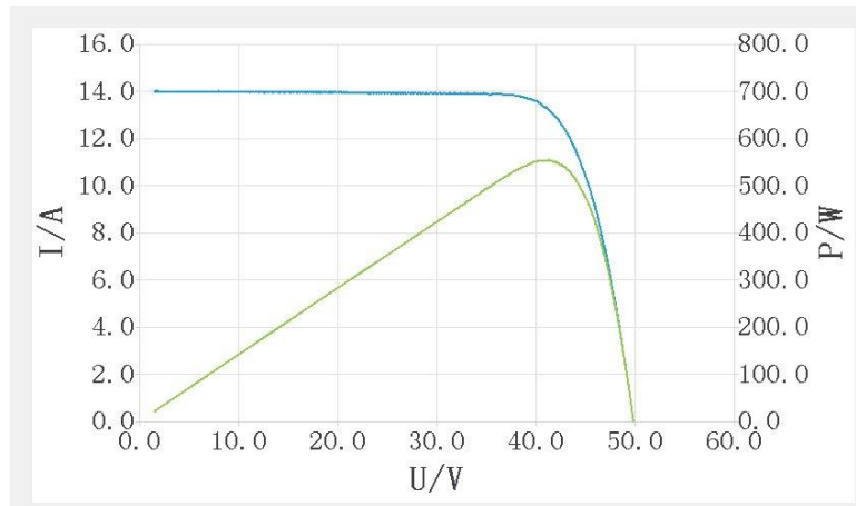
Fig. 6 IV curve of module No.2 Serial number: AS22191106795
