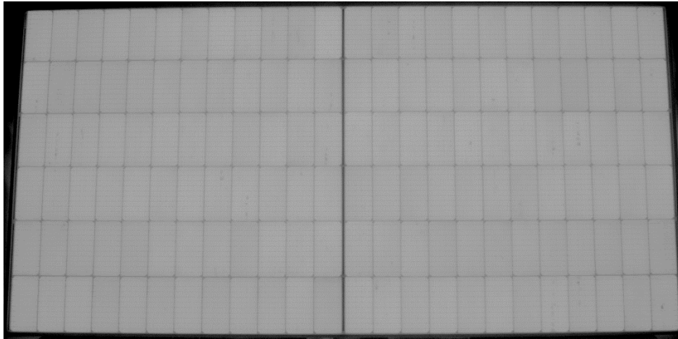
Fig. 8 EL photo of module No.2 Serial number: AS22191106795
